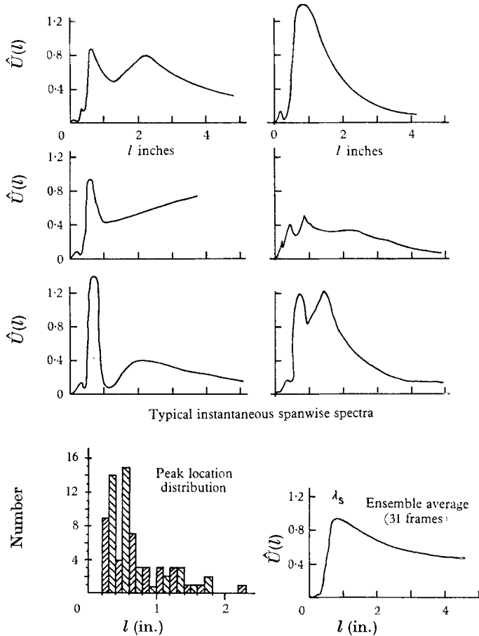
FIGURE 14. Typical instantaneous and average spanwise spectra. dP/dx \gg 0 , y^+ \approx 2 .
