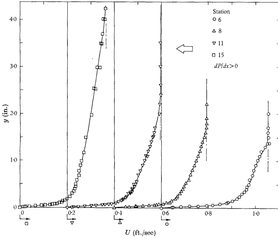
FIGURE 7b. Mean profiles for the mild positive pressure gradient flow.
