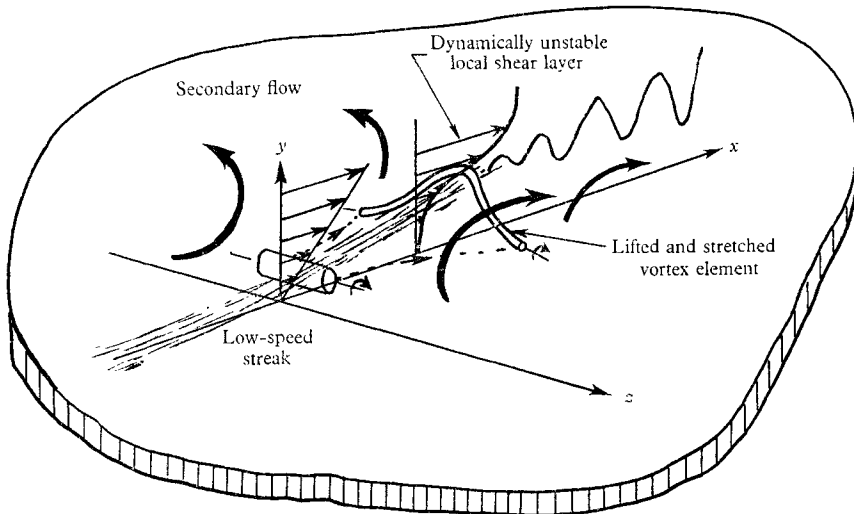
FIGURE 19b. The mechanics of streak breakup.
