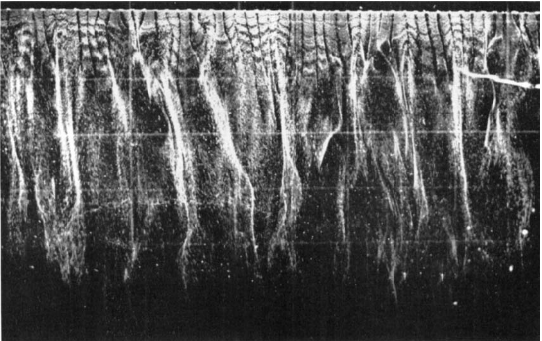
FIGURE 10 b. y^+ = 4.5 .
