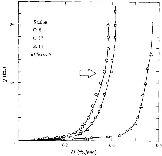
FIGURE 7e. Mean profiles for the strong negative pressure gradient flow.
