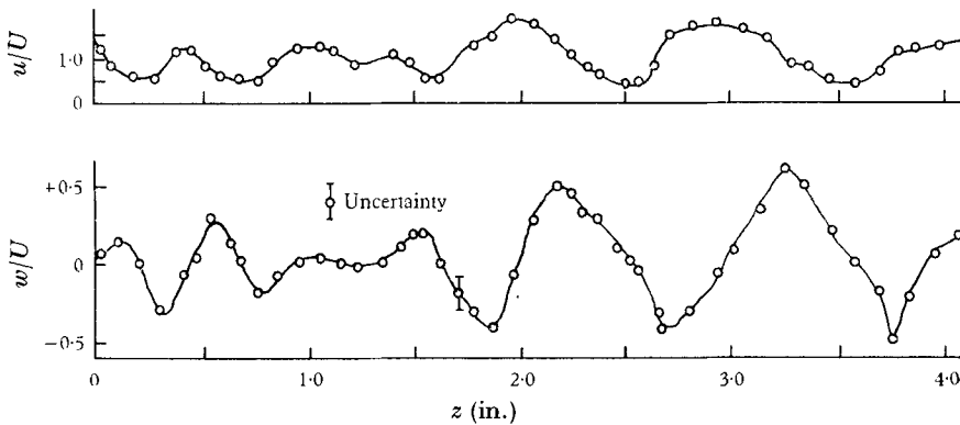
FIGURE 13. Typical instantaneous spanwise variation in u and w , determined by the bubble marker method ( y^+ \approx 5 ).
