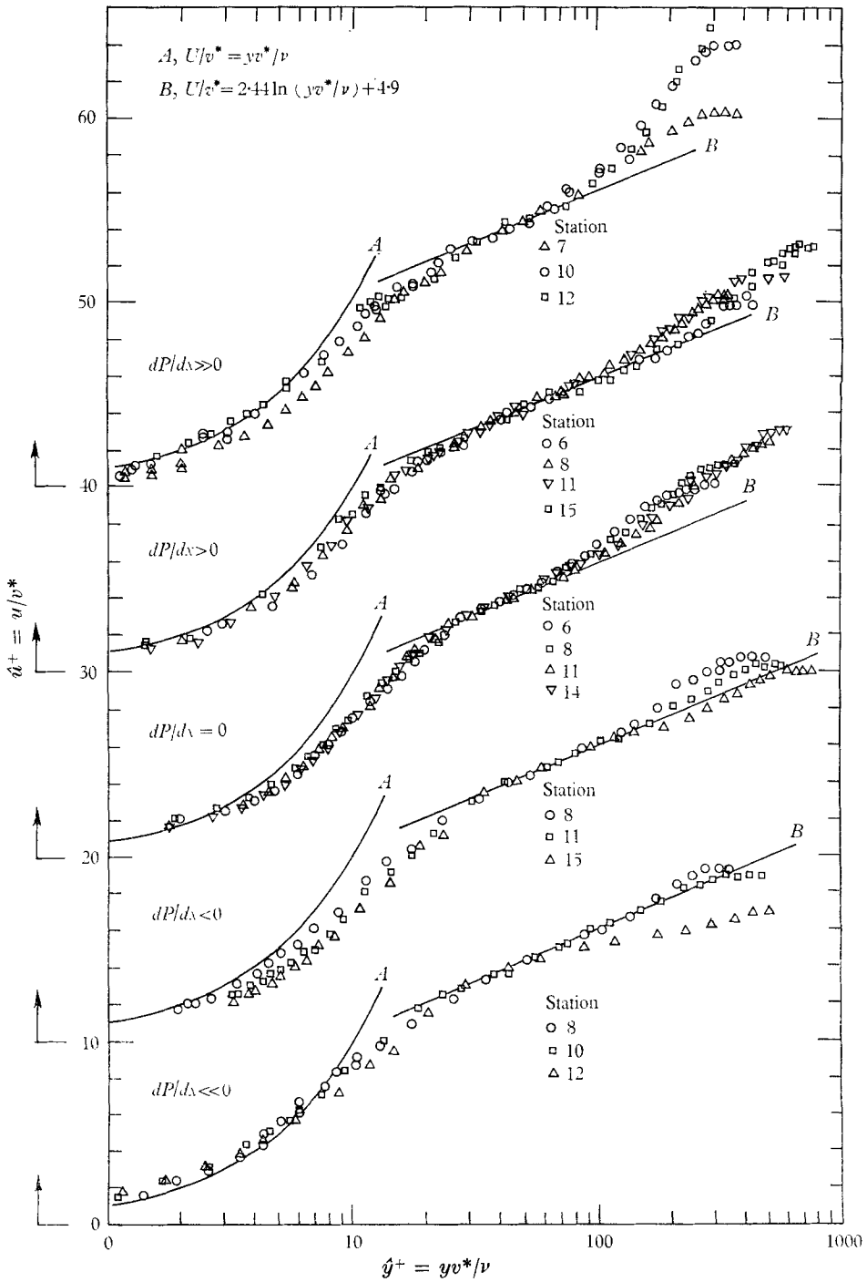
FIGURE 9a. u^+ - \hat{y}^+ profiles using v^* (note shifted origins).
