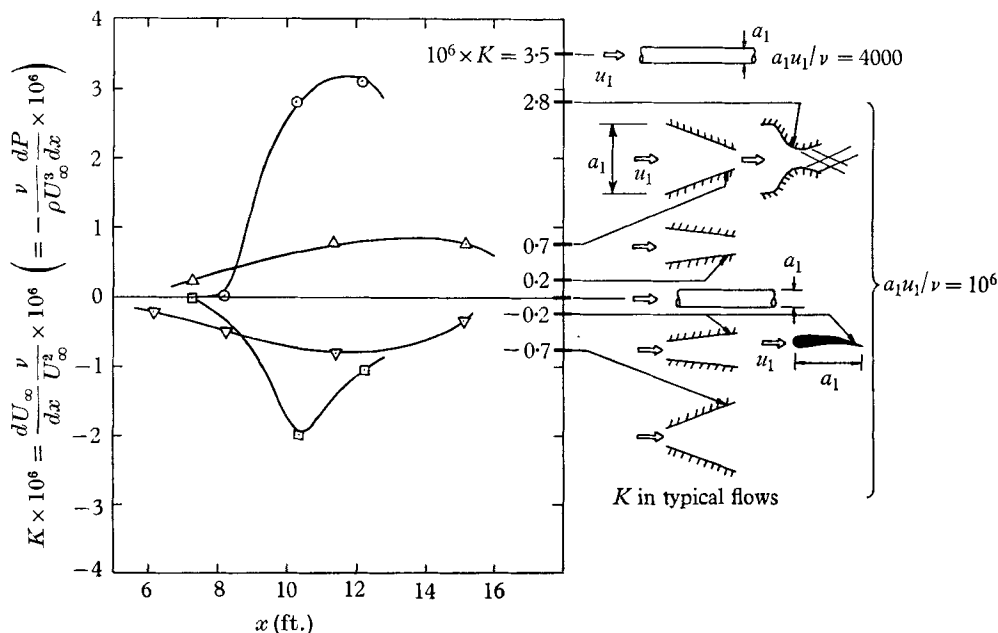
FIGURE 6b. Pressure gradient parameter distributions. \circ , dP/dx \ll 0 ; \triangle , dP/dx < 0 ; \nabla , dP/dx > 0 ; \square , dP/dx \gg 0 .
