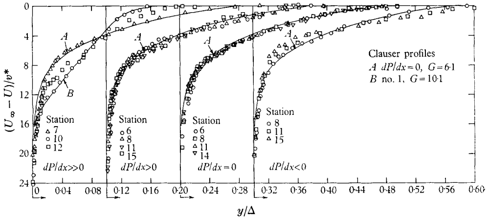
FIGURE 8. Velocity defect profiles.
