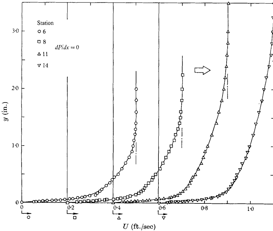
FIGURE 7c. Mean profiles for the zero pressure gradient flow.
