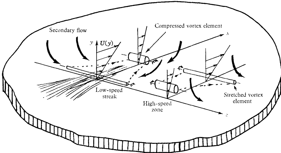
FIGURE 19a. The mechanics of streak formation.
