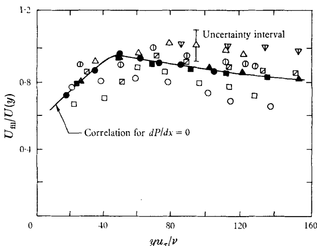
FIGURE 18. Average velocities of ejected eddies.
