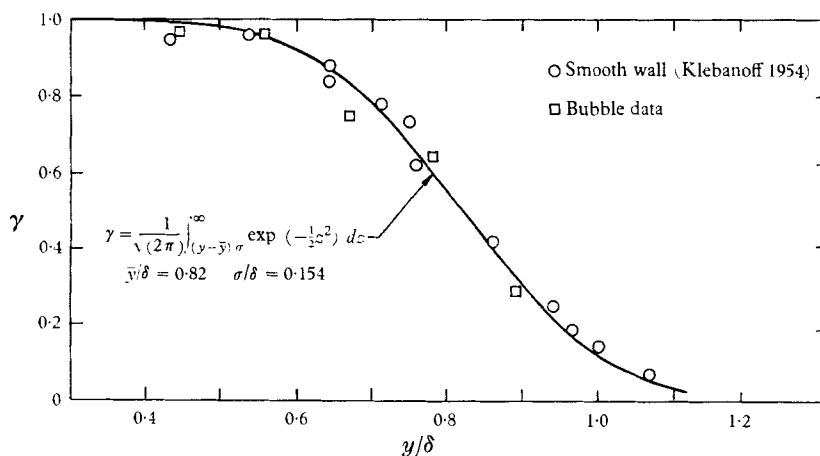
FIGURE 11. Intermittency distribution by the bubble technique.
