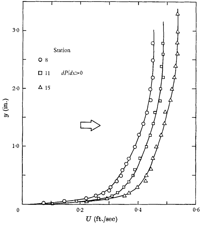
FIGURE 7d. Mean profiles for the mild negative pressure gradient flow.
