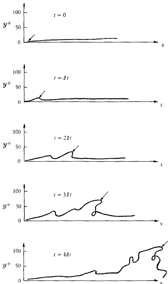
FIGURE 15. Dye streak breakup; illustration as seen in side view.
