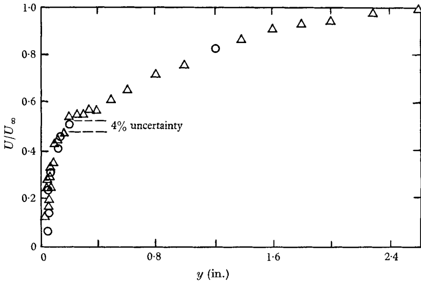
FIGURE 3b. Comparison of mean velocity data from hot-wire and bubble techniques. Station 10, dP/dx \gg 0 . \Delta , hot wire; \circ , hydrogen bubble.
