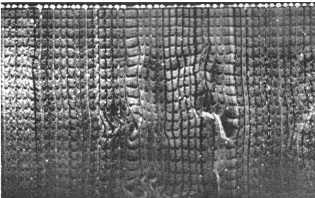
FIGURE 10 h . y^+ = 507 .
