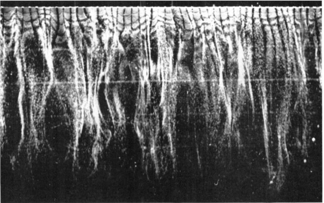
FIGURE 10 a. y^+ = 2.7 .
