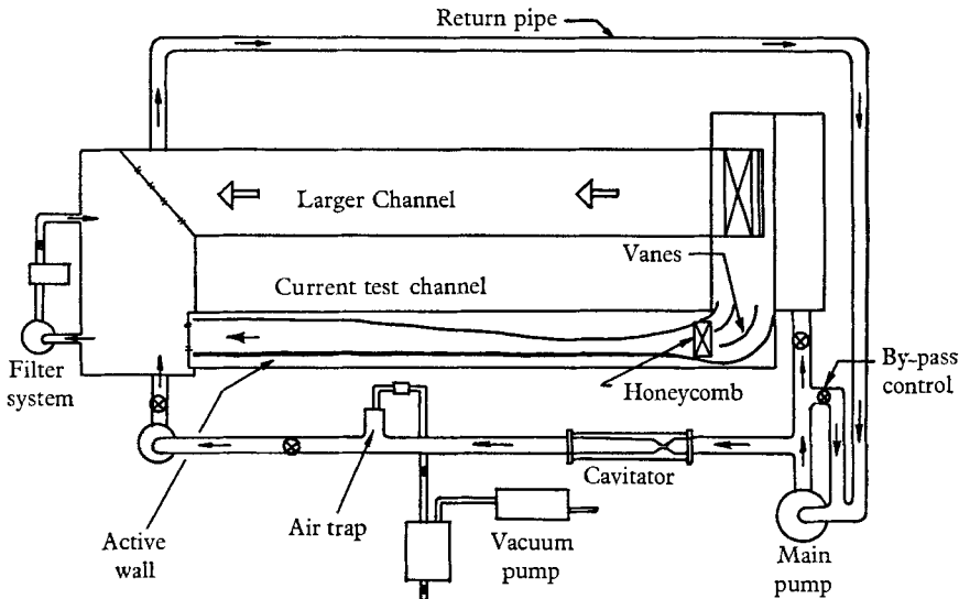
FIGURE 2. Flow system.
