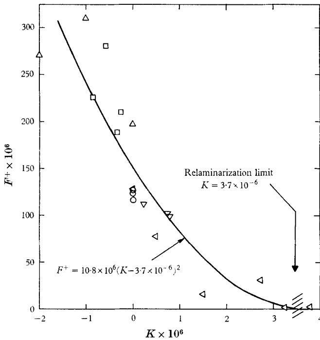
FIGURE 16b. Normalized burst rate as a function of K . \triangle , dP/dx > 0 ; \square , dP/dx > 0 ; \circ , dP/dx = 0 ; \nabla , dP/dx < 0 ; \triangleleft , dP/dx \leq 0 .
