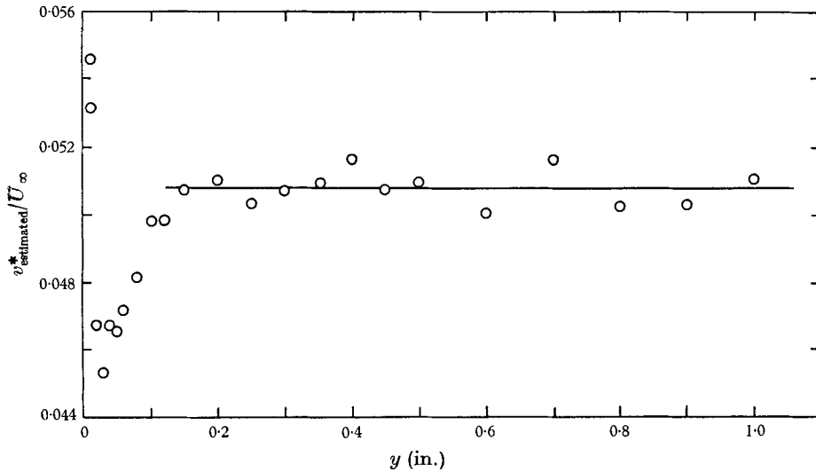
FIGURE 5b. Determination of the wall shear stress by the cross-plot method. Station 6, dP/dx < 0 . v^*/U_{\infty} = 0.0508 , U_{\infty} = 0.462 ft./sec; v^* = 0.023 ft./sec.
