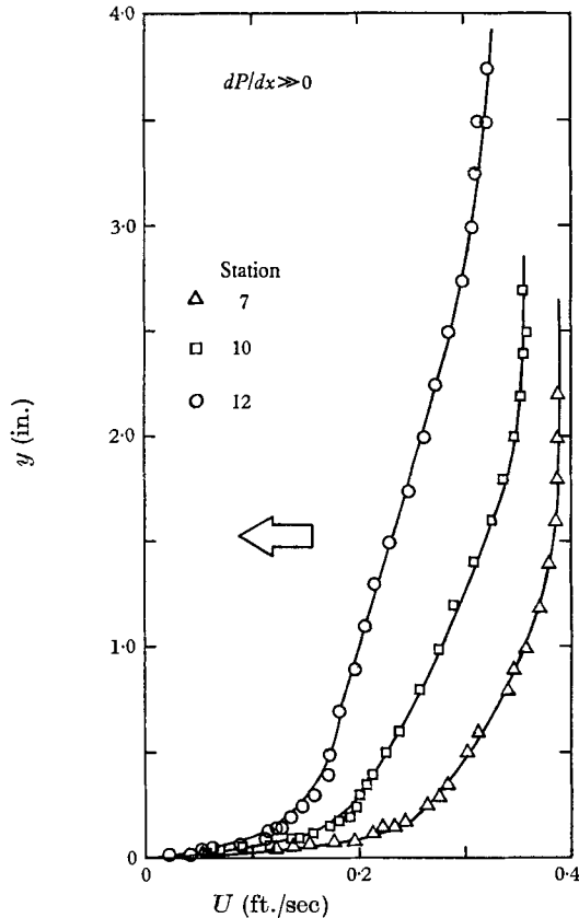
FIGURE 7a. Mean profiles for the strong positive pressure gradient flow.
