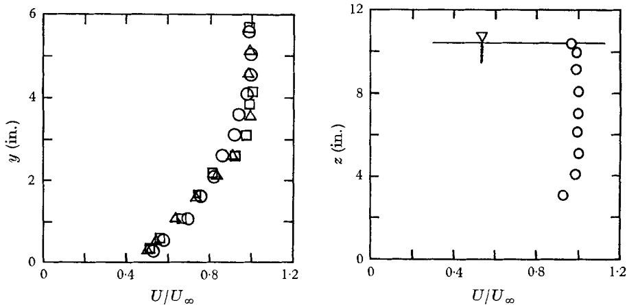
FIGURE 4. Representative checks on the two-dimensionality of the flow. Station 12, dP/dx \geq 0 (worst case), y = 4.50 in. \circ , z = 10 in.; \triangle , z = 7.7 in.; \square , z = 5.5 in.
