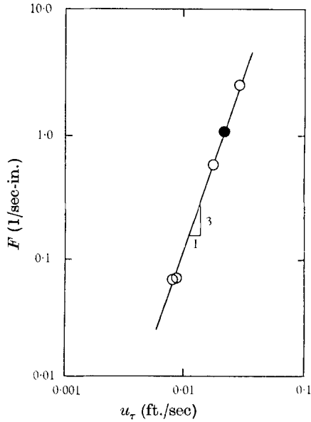
FIGURE 16a. Burst rate as a function of shear velocity. dP/dx = 0 ; \circ , Runstadler et al. (1963), 3 velocities; \bullet , present data, 3 x stations.
