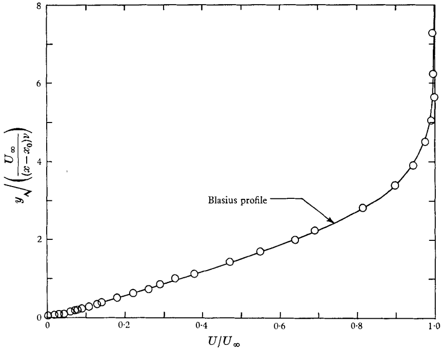
FIGURE 3a. Test of the hot wire in a laminar flow. \circ , hot-wire data; x_0 , effective origin found by fit.
