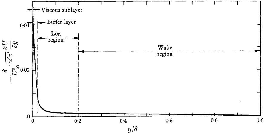
FIGURE 1a. Normalized turbulence energy production rate per unit volume in a typical boundary layer (Klebanoff 1954).
