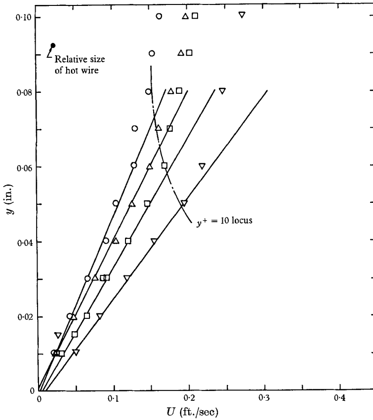
FIGURE 5a. Determination of the wall shear stress by the wall-slope method. \nabla , station 6; \square , station 8; \Delta , station 11; \circ , station 15; dP/dx < 0 .
