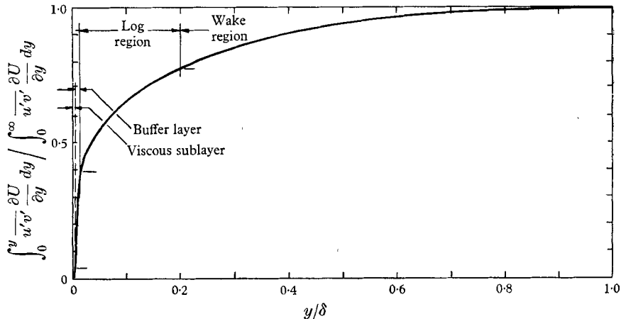
FIGURE 1b. Cumulative turbulence energy production rate in a typical turbulent boundary layer (Klebanoff 1954).
