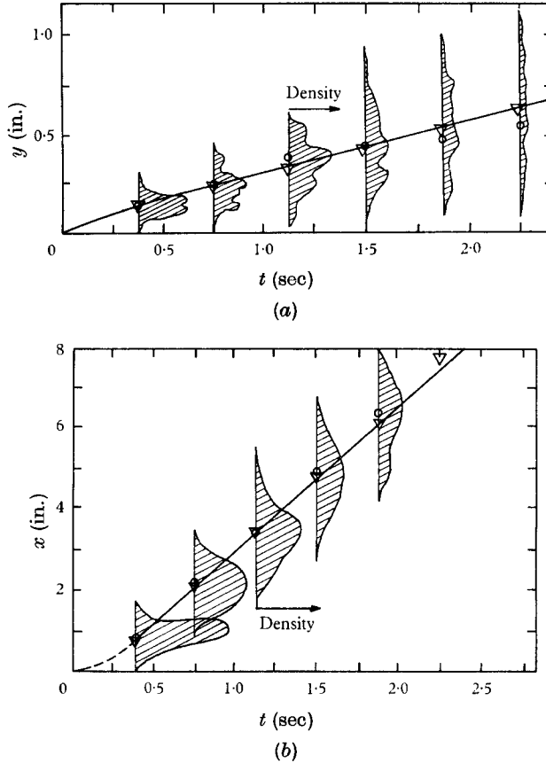
FIGURE 17. Trajectories of ejected eddies—flat plate flow. Station 10, dP/dx = 0 ; \nabla , averages; \circ , maxima.
