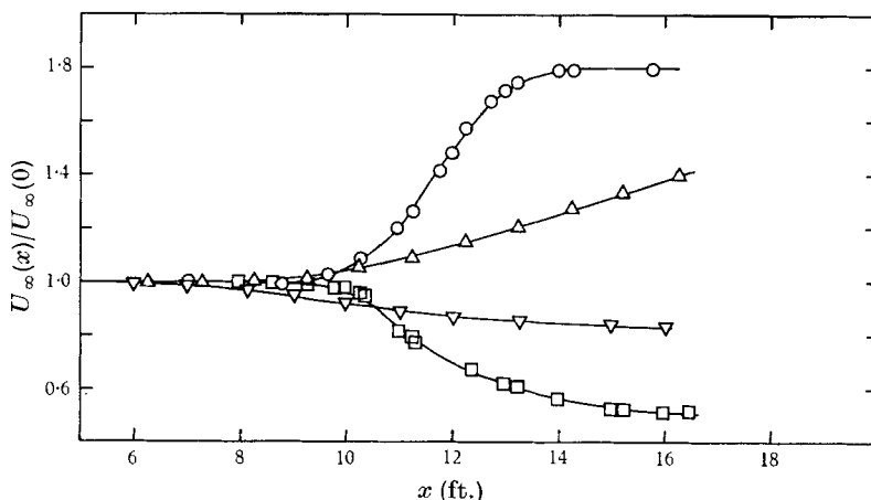
FIGURE 6a. Free-stream velocity distributions. \circ , dP/dx \ll 0 ; \triangle , dP/dx < 0 ; \nabla , dP/dx > 0 ; \square , dP/dx \gg 0 .
